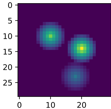
Noise-less data
